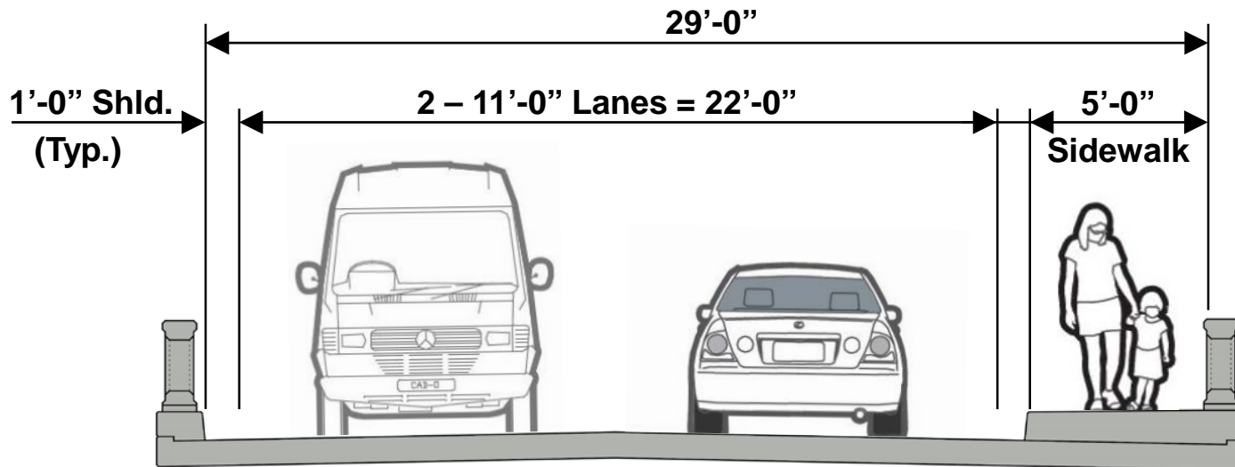
SIDEWALK WITH 1' SHOULDERS
