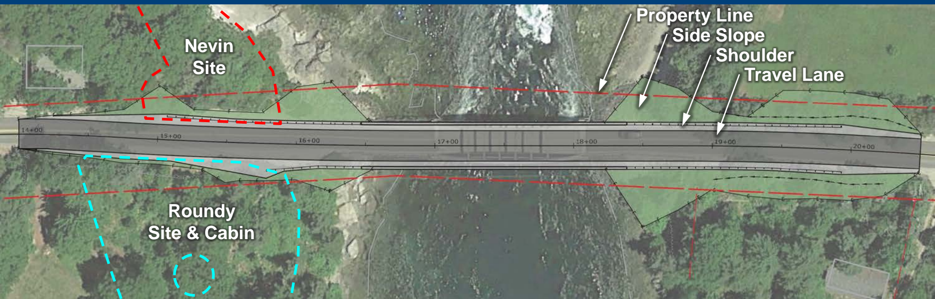
PLAN LAYOUT (Option with Widened Shoulders Shown)
