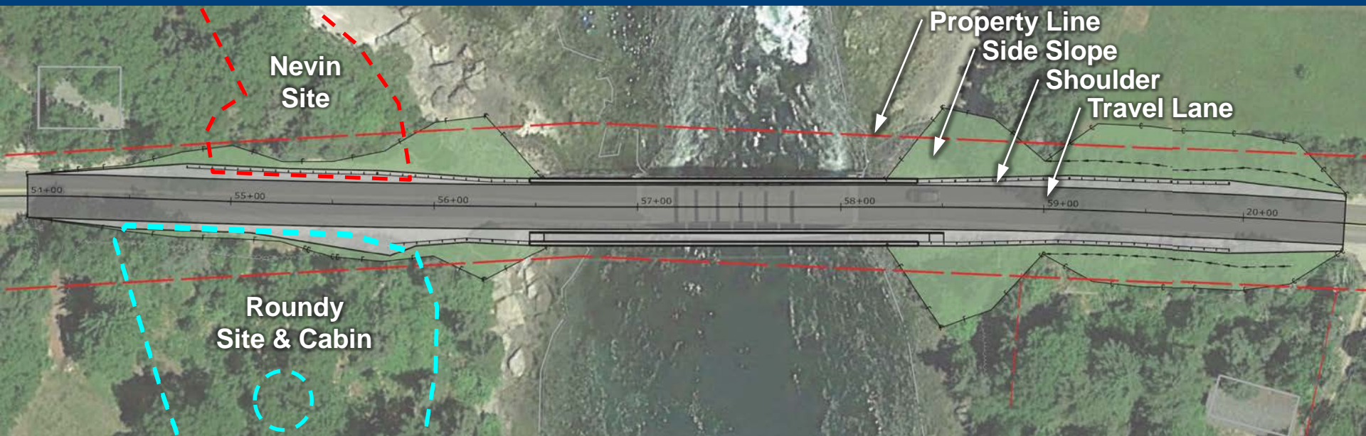
PLAN LAYOUT (Option with Sidewalk Shown)
